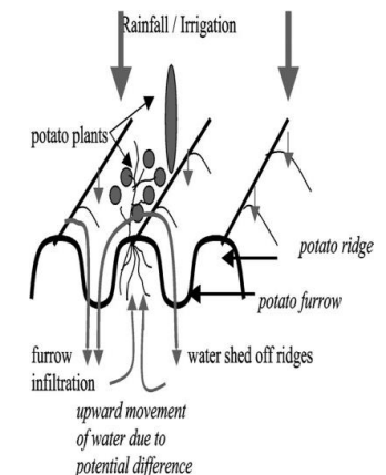
Water relations with a raised bed system
