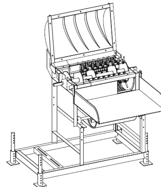
Axial flow principle
