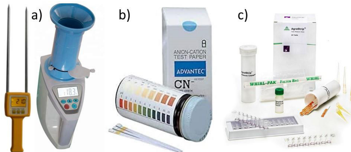
Examples of a) flour moisture meters and b) cyanide and c) aflatoxin qualitative test kits
